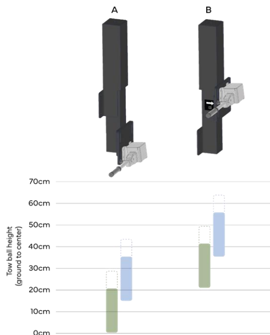
Figure 4. Height adjustment tower rotation
